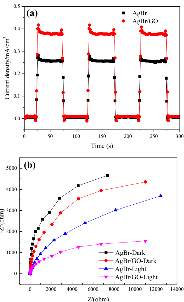
Fig. 6 Transient photocurrent response (a) and EIS curves (b) of AgBr and AgBr/GO nano-catalysts
