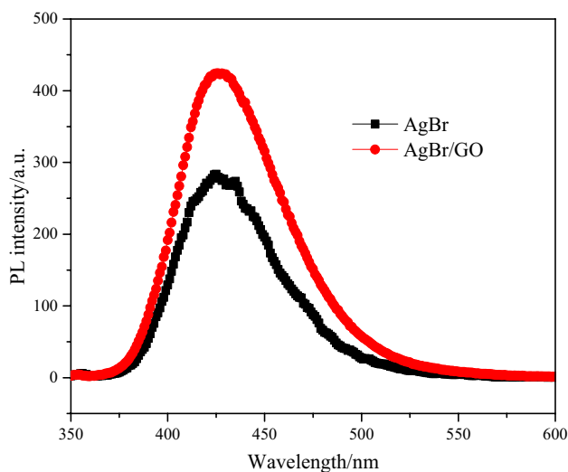
Fig. 7 Fluorescence spectra of AgBr and AgBr/GO nano-catalysts
