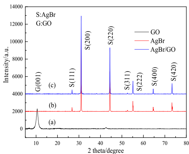
Fig. 2 XRD patterns of pristine GO (a), AgBr (b) and AgBr/GO (c) nano-catalysts
