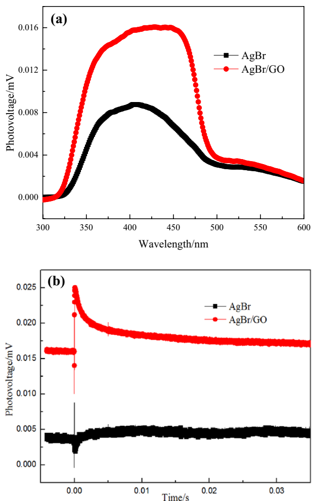
Fig. 5 Surface photovoltage (a) and time-resolved surface photovoltage (b) responses of AgBr and AgBr/GO nano-catalysts
