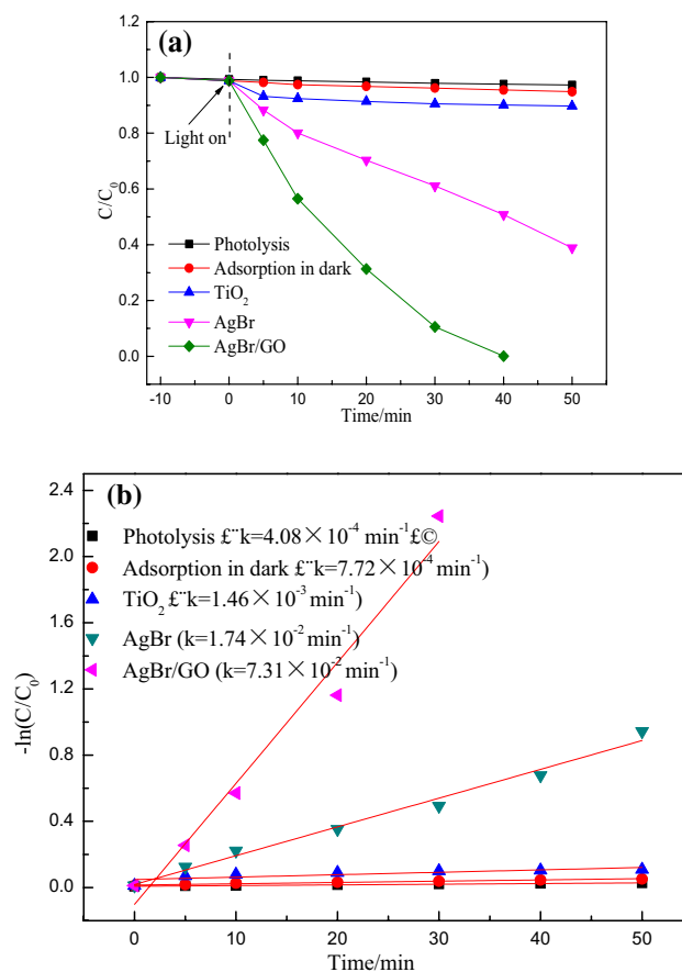
Fig. 8 Photocatalytic degradation of PCBA (a) under simulated sun-light irradiation; kinetic linear fitting curves of \ln(C_0/C) versus degradation time for PCBA (b) by as-prepared nano-catalysts
