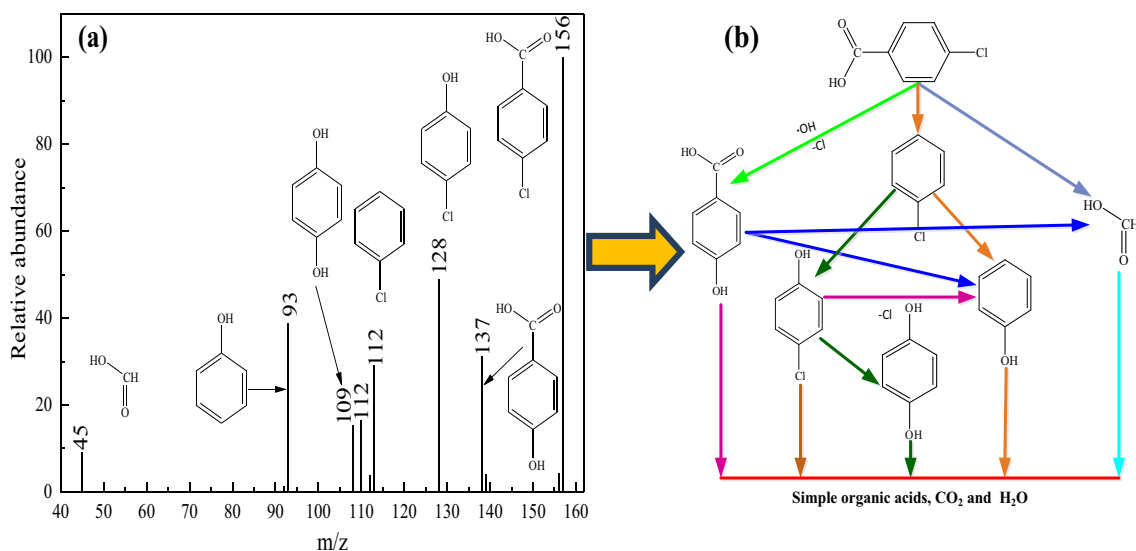
Fig. 10 Proposed decomposition pathways of PCBA in the AgBr/GO nanocomposites
