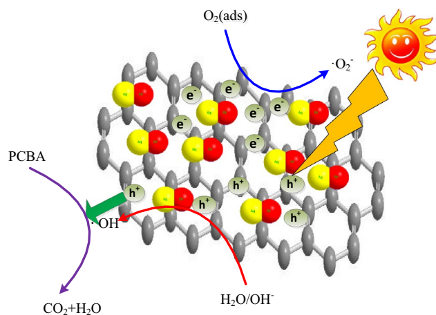
Fig. 9 Scheme of PC mechanism for AgBr/GO nano-catalysts
