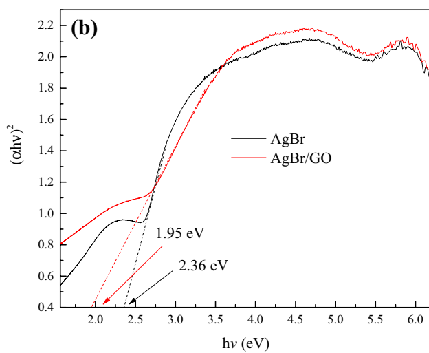
Fig. 4 UV-Vis DRS absorption spectra of AgBr and AgBr/GO nano-catalysts
