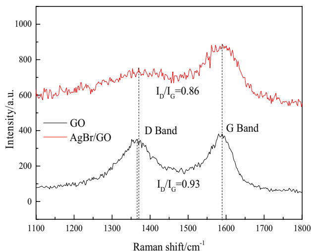
Fig. 3 Raman spectroscopy of GO and AgBr/GO nano-catalysts
